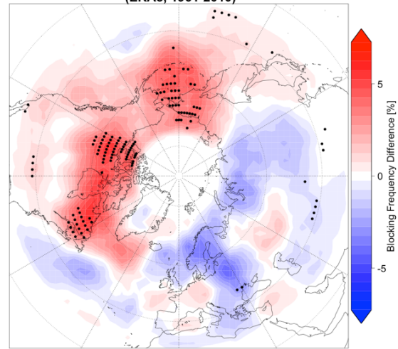
Spring BF Difference between High and Low AMV Years (ERA5, 1961-2010)
