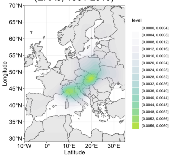
Vb Density Function in Combination with Eastern Europe and Scandinavian Block (ERA5, 1961-2010)
