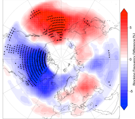
Jan-March BF Difference between High and Low November Snow Cover Difference Years (IPSL-CM6A-LR, SSP5-8.5, 2051-2100)
