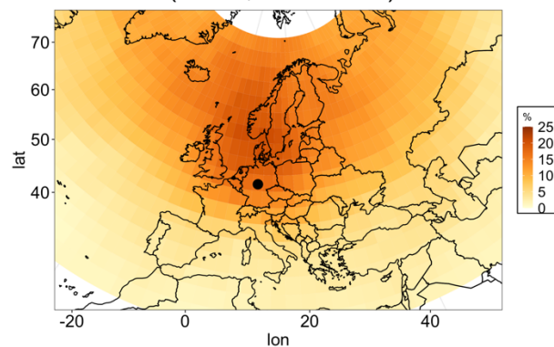
Frequency of Blocking during Calm (ERA5, 1961-2010)
