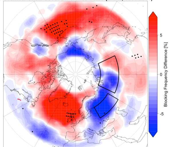
January-March BF Difference between High and Low AMV & November Snow Cover Difference Years (ERA5, 1961-2010)
