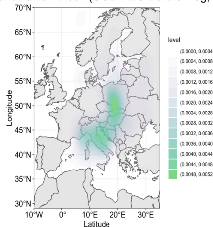
Vb Density Function in Combination with Eastern Europe and Scandinavian Block (CCLM-EC-Earth3-Veg, 1961-2010)
