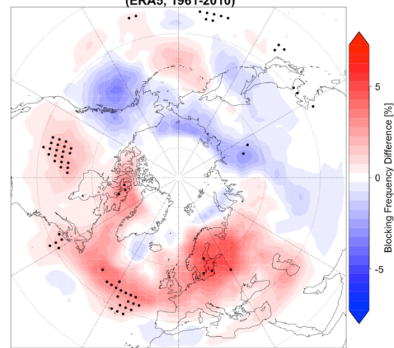
Autumn BF Difference between High and Low AMV Years (ERA5, 1961-2010)
