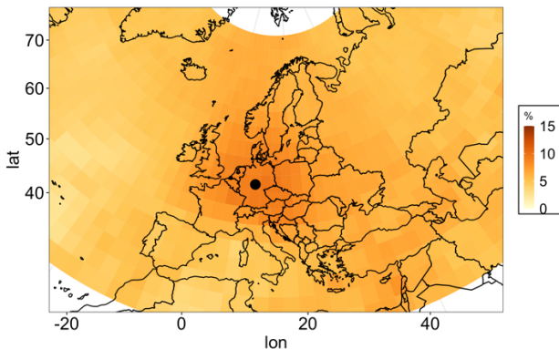
Frequency of Calm in Case of Blocking (ERA5, 1961-2010)
