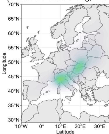
Vb Density Function without Blocking (CCLM-EC-Earth3-Veg, 2051-2099)
