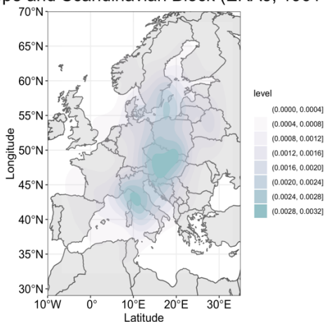
Vb Density Function in Combination with Eastern Europe and Scandinavian Block (ERA5, 1961-2010)
