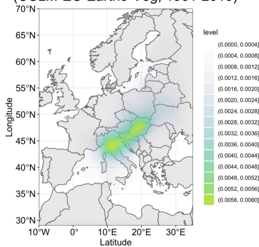
Vb Density Function in Combination with Eastern Europe and Scandinavian Block (CCLM-EC-Earth3-Veg, 1961-2010)
