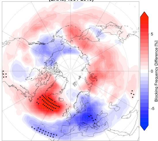
Winter BF Difference between High and Low AMV Years (ERA5, 1961-2010)
