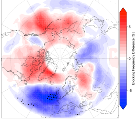
Jan-March BF Difference between High and Low November Snow Cover Difference Years (CNRM-CM6-1, SSP5-8.5, 2051-2100)
