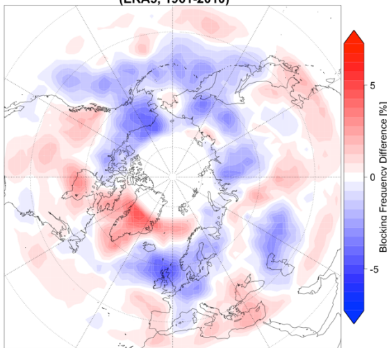
Summer BF Difference between High and Low AMV Years (ERA5, 1961-2010)
