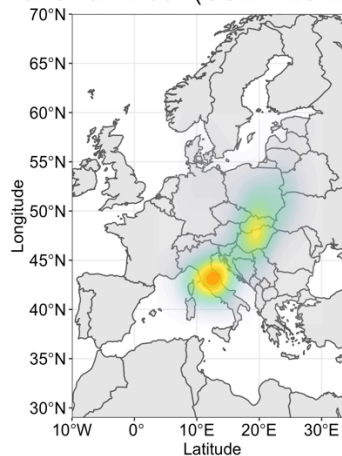
Vb Density Function in Combination with Eastern Europe and Scandinavian Block (CCLM-EC-Earth3-Veg, 2051-2099)
