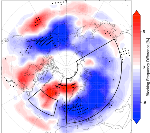
Spring BF Difference between High and Low March EUR Snow Cover & NA SST Anomaly Years (ERA5, 1961-2010)
